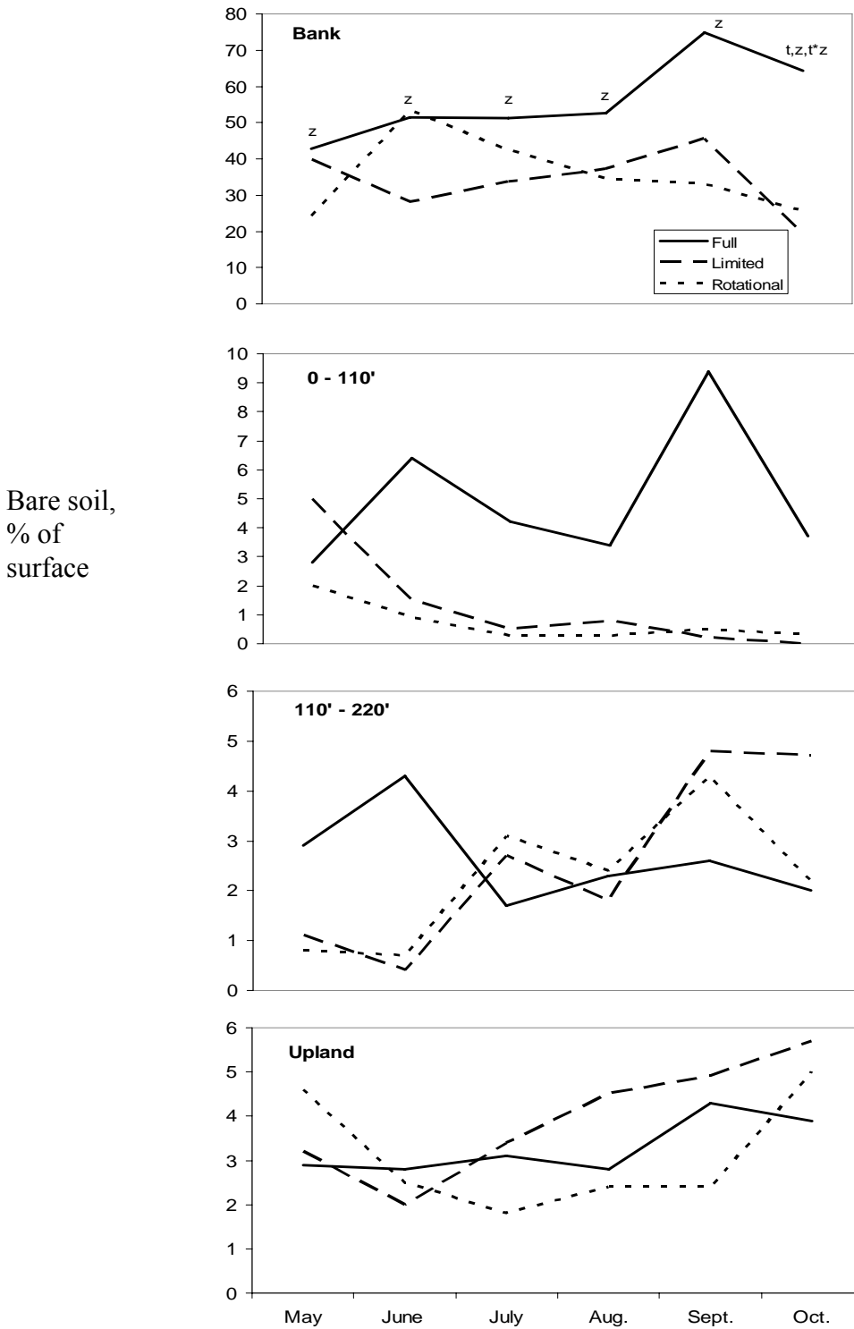
Figure 1. Least squares means of the proportion of soil surface that was bare, weighted for congregation and open areas, in different zones of pastures with continuous grazing and full or limited stream access or rotational grazing. (t, z and t*z designate significant treatment effects, zone effects, and treatment by zone interactions, P < 0.05).
